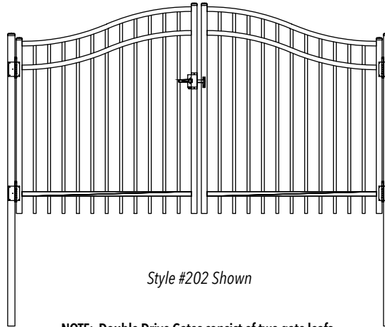
ARCHED ESTATE GATE DIMENSIONAL DRAWING
